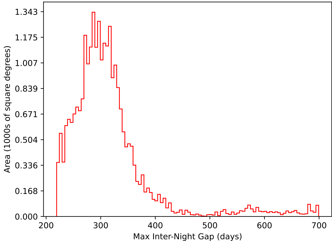
too_elab_2yr_r128_d3_ugrizy_v3.4_10yrs All sky i band: Max Inter-Night Gap
