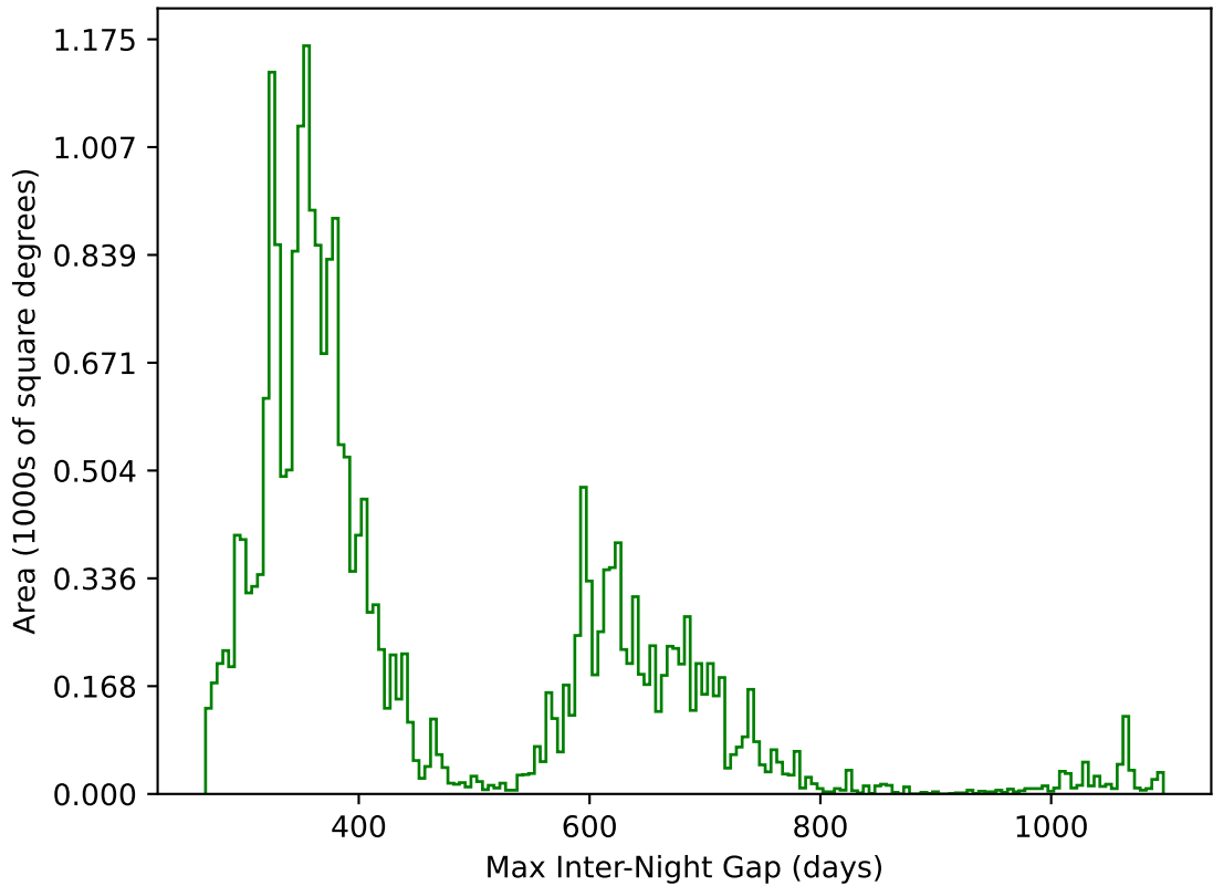
too_elab_2yr_r128_d3_ugrizy_v3.4_10yrs All sky g band: Max Inter-Night Gap
