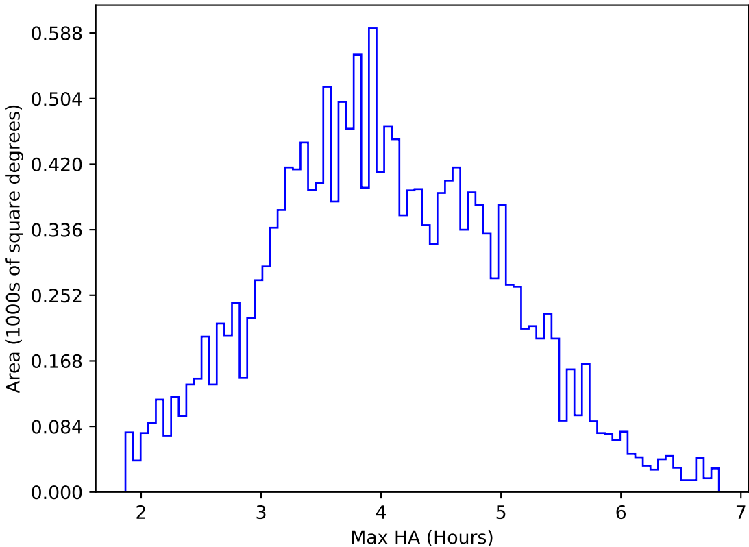
too_elab_2yr_r128_d3_ugrizy_v3.4_10yrs WFD u band: Max HA
