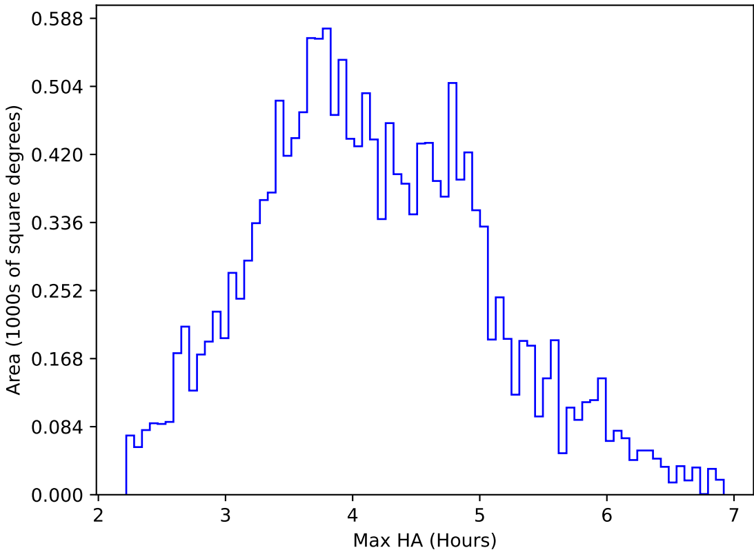
too_elab_2yr_r128_d3_ugrizy_v3.4_10yrs WFD g band: Max HA
