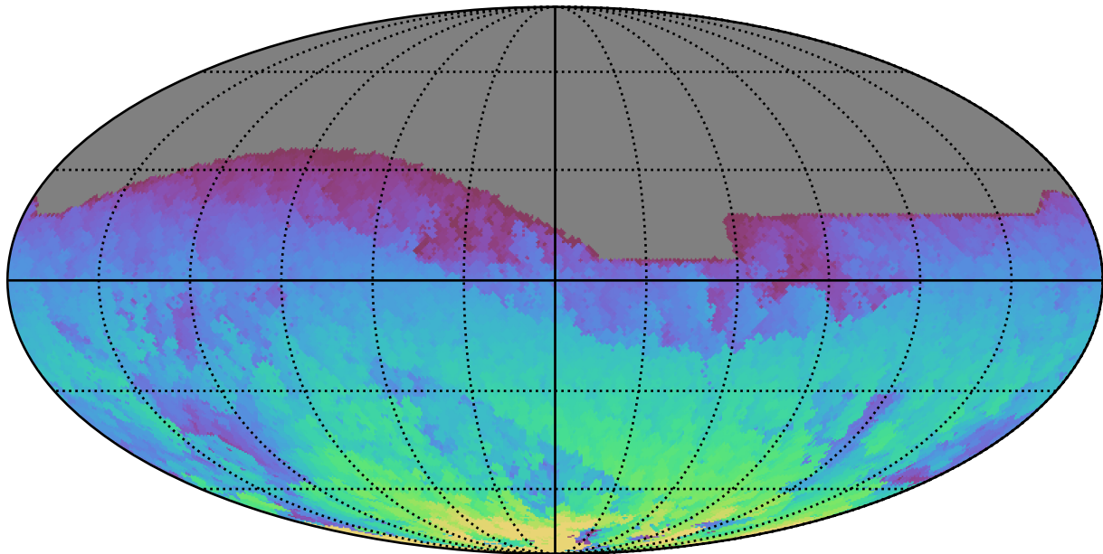
too_elab_2yr_r128_d3_ugrizy_v3.4_10yrs All sky z band: Max HA
