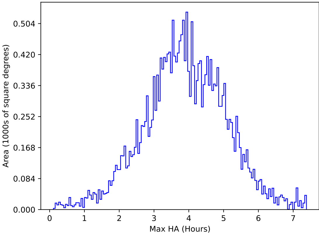
too_elab_2yr_r128_d3_ugrizy_v3.4_10yrs All sky u band: Max HA
