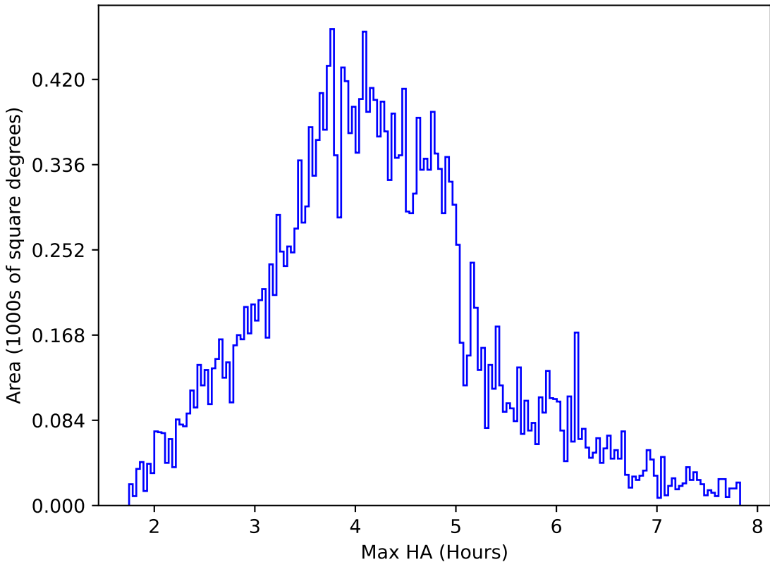
too_elab_2yr_r128_d3_ugrizy_v3.4_10yrs All sky r band: Max HA
