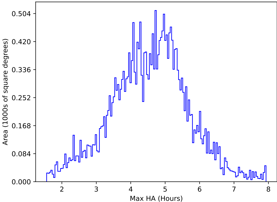
too_elab_2yr_r128_d3_ugrizy_v3.4_10yrs All sky i band: Max HA
