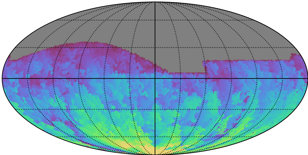
too_elab_2yr_r128_d3_ugrizy_v3.4_10yrs All sky g band: Max HA
