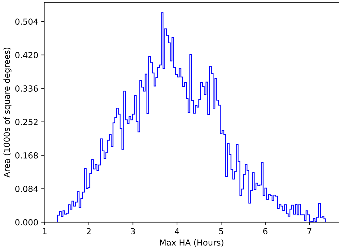
too_elab_2yr_r128_d3_ugrizy_v3.4_10yrs All sky g band: Max HA
