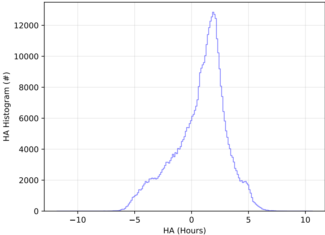
too_elab_2yr_r128_d3_ugrizy_v3.4_10yrs WFD z band: HA Histogram
