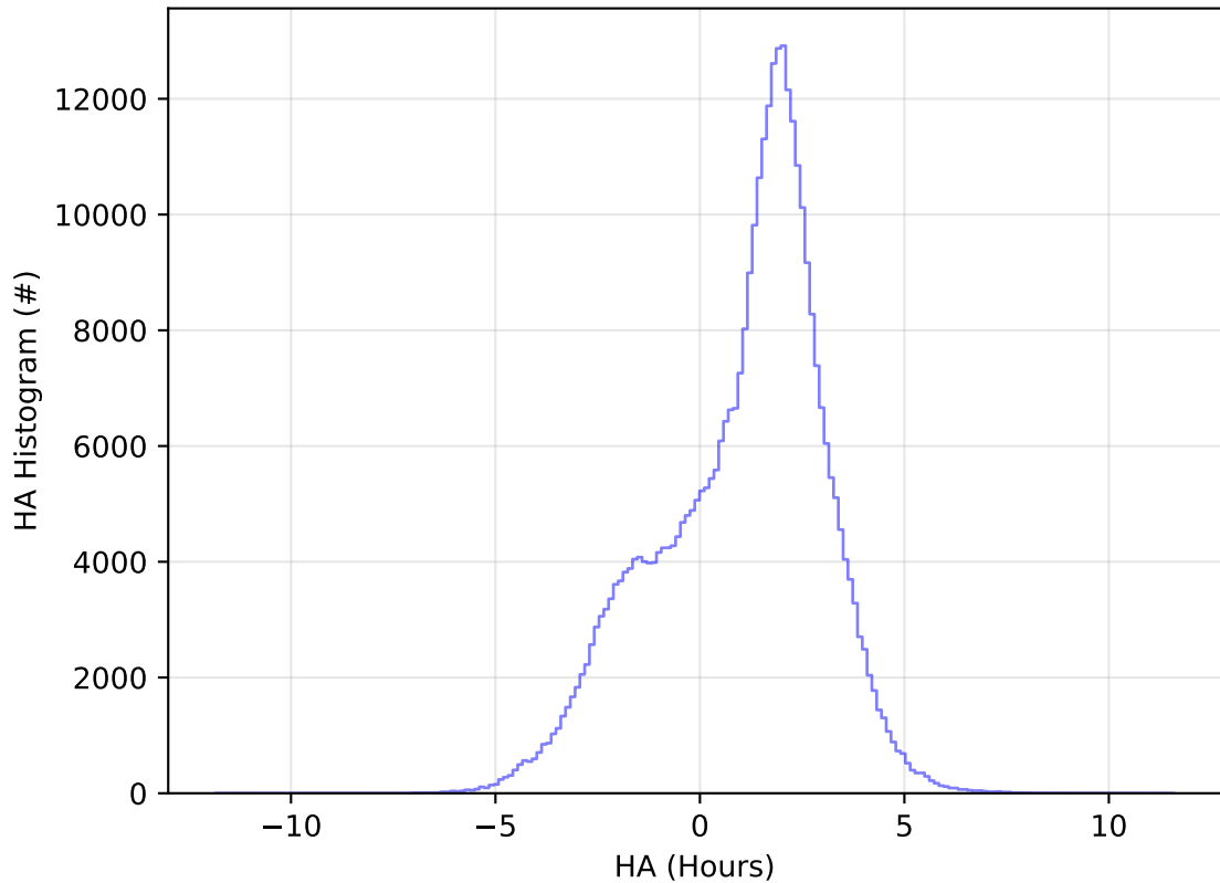
too_elab_2yr_r128_d3_ugrizy_v3.4_10yrs WFD y band: HA Histogram
