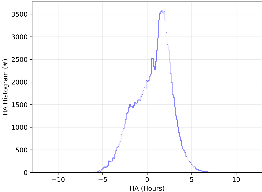
too_elab_2yr_r128_d3_ugrizy_v3.4_10yrs WFD u band: HA Histogram
