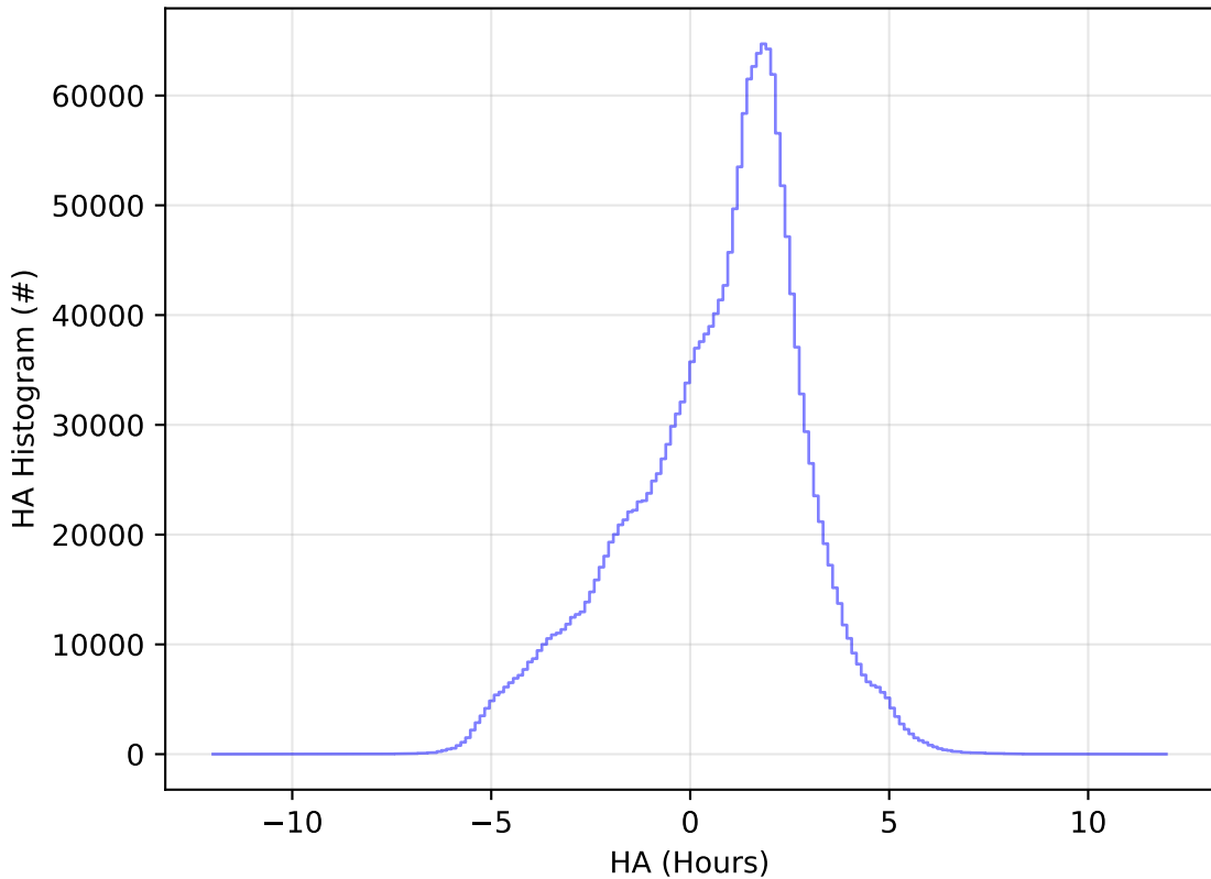
too_elab_2yr_r128_d3_ugrizy_v3.4_10yrs WFD all bands: HA Histogram
