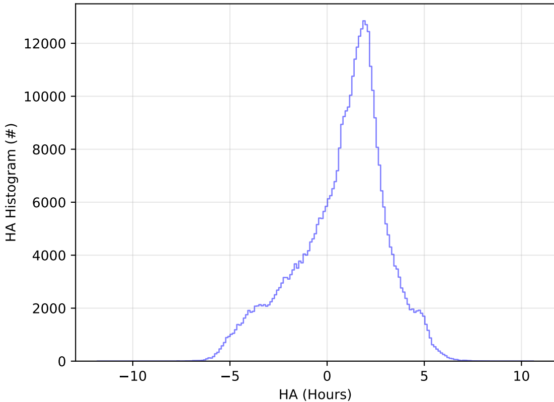
too_elab_2yr_r128_d3_ugrizy_v3.4_10yrs All sky z band: HA Histogram
