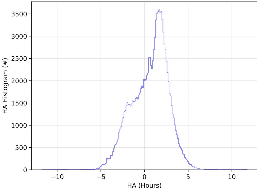
too_elab_2yr_r128_d3_ugrizy_v3.4_10yrs All sky u band: HA Histogram
