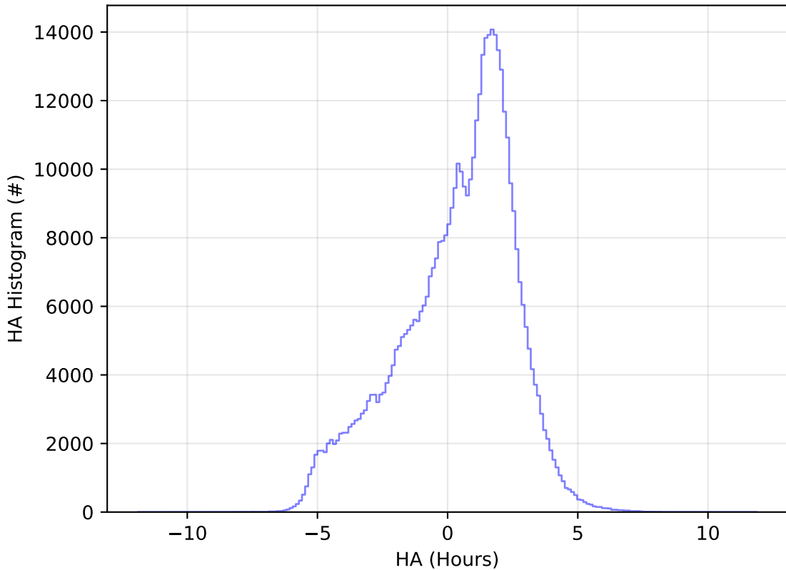
too_elab_2yr_r128_d3_ugrizy_v3.4_10yrs All sky r band: HA Histogram
