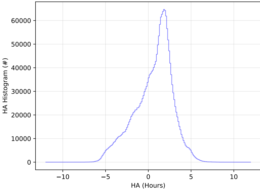
too_elab_2yr_r128_d3_ugrizy_v3.4_10yrs All sky all bands: HA Histogram
