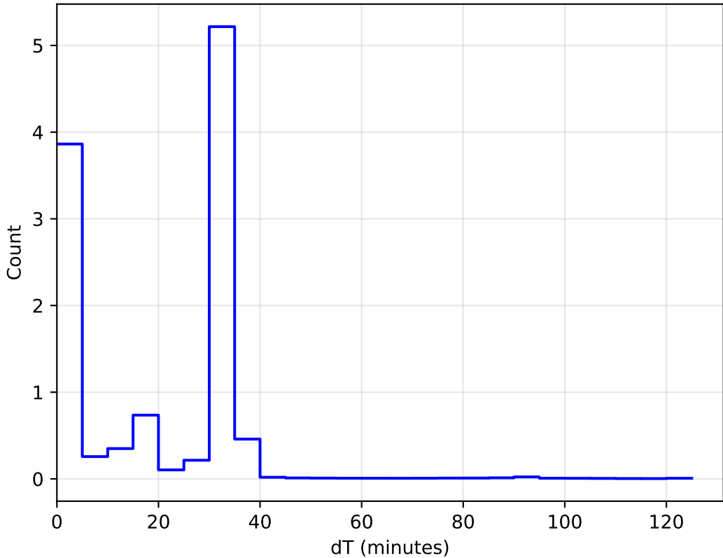
too_elab_2yr_r128_d3_ugrizy_v3.4_10yrs WFD: DeltaT Histogram 1e6
