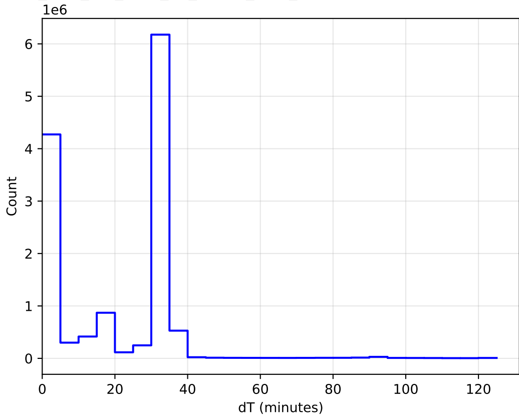
too_elab_2yr_r128_d3_ugrizy_v3.4_10yrs All sky: DeltaT Histogram
