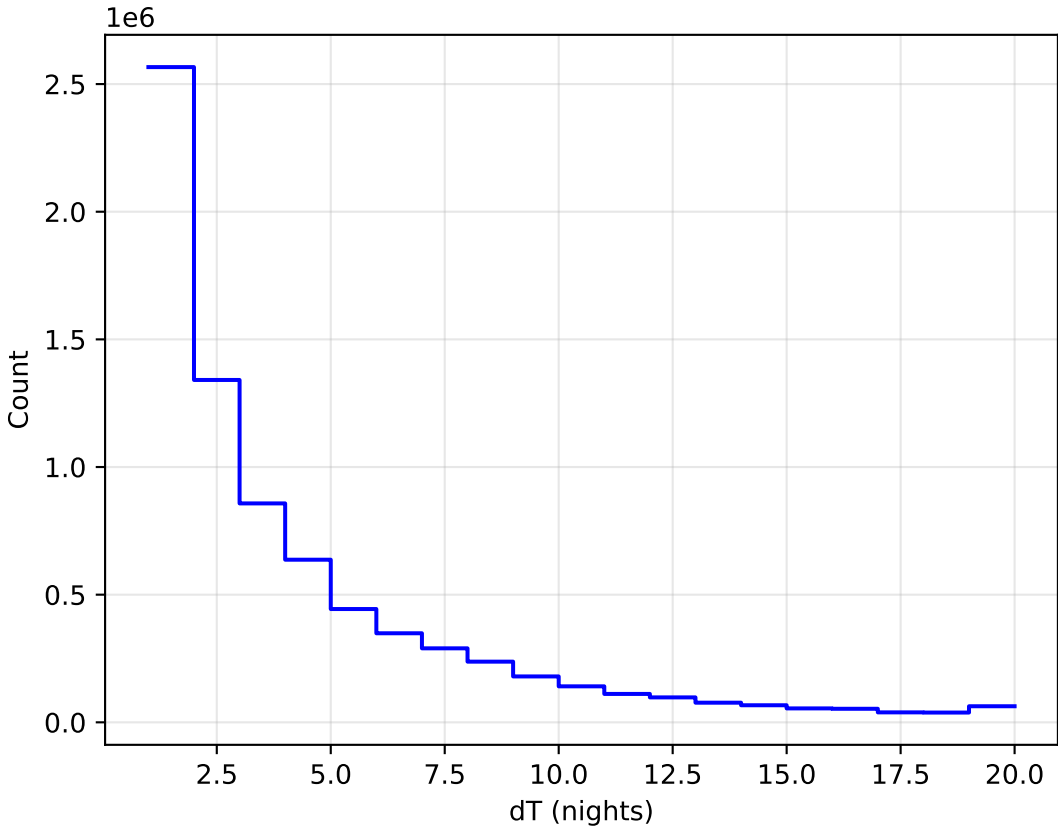
too_elab_2yr_r128_d3_ugrizy_v3.4_10yrs WFD all bands: DeltaNight Histogram
