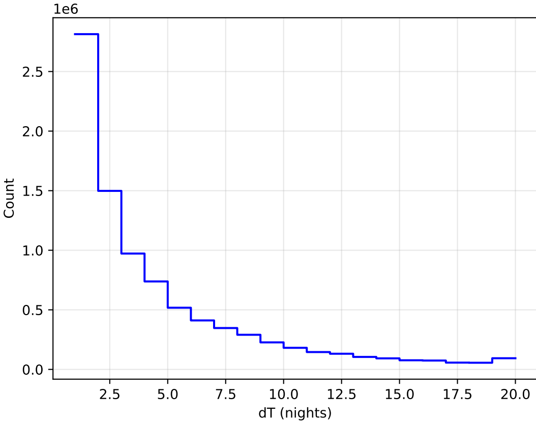
too_elab_2yr_r128_d3_ugrizy_v3.4_10yrs All sky all bands: DeltaNight Histogram
