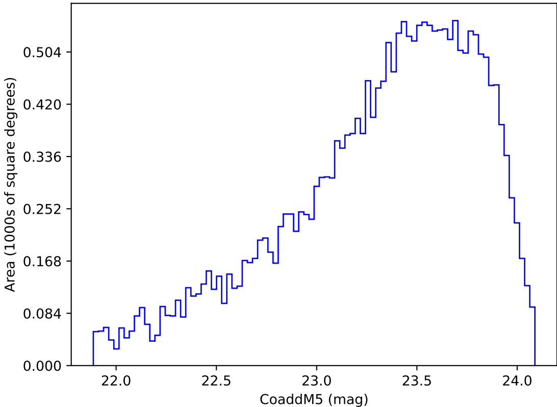
too_elab_2yr_r128_d3_ugrizy_v3.4_10yrs Yr 3-4 y band: CoaddM5
