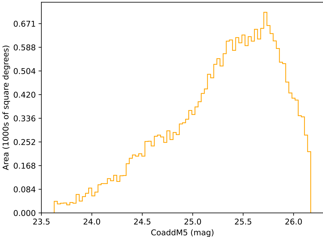
too_elab_2yr_r128_d3_ugrizy_v3.4_10yrs Yr 3-4 r band: CoaddM5
