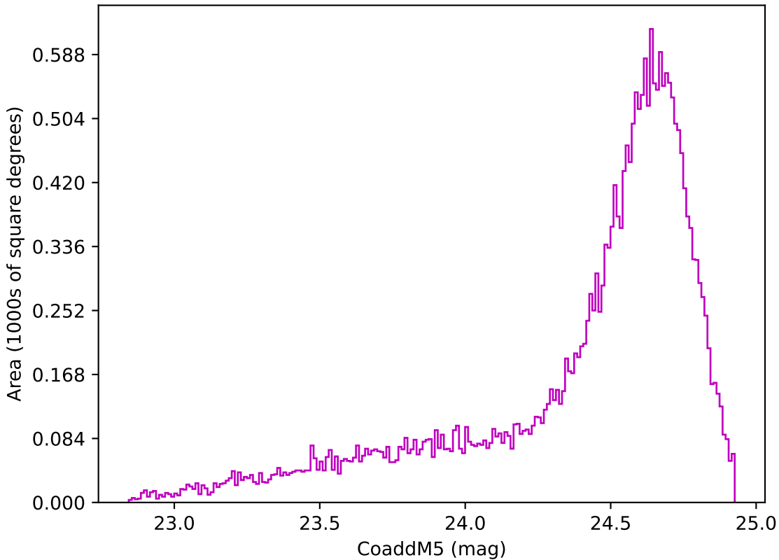
too_elab_2yr_r128_d3_ugrizy_v3.4_10yrs Yr 1 z band: CoaddM5
