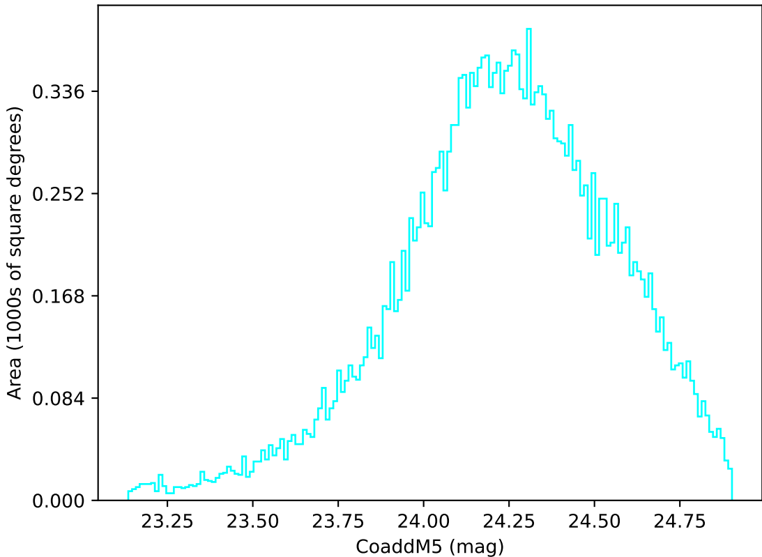
too_elab_2yr_r128_d3_ugrizy_v3.4_10yrs Yr 1 u band: CoaddM5
