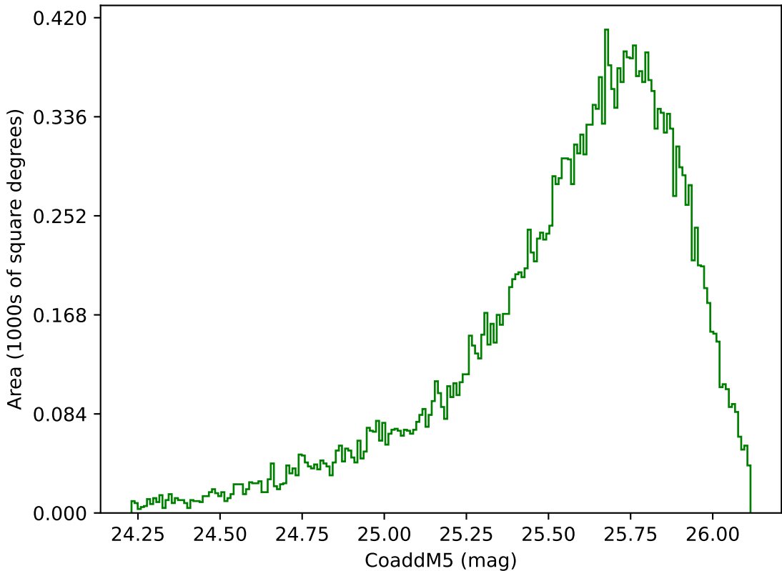
too_elab_2yr_r128_d3_ugrizy_v3.4_10yrs Yr 1 g band: CoaddM5
