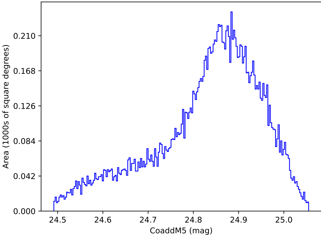
too_elab_2yr_r128_d3_ugrizy_v3.4_10yrs WFD y band: CoaddM5
