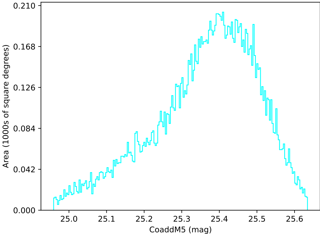
too_elab_2yr_r128_d3_ugrizy_v3.4_10yrs WFD u band: CoaddM5
