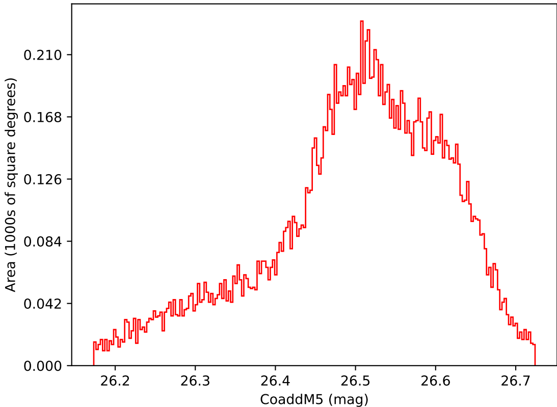
too_elab_2yr_r128_d3_ugrizy_v3.4_10yrs WFD i band: CoaddM5
