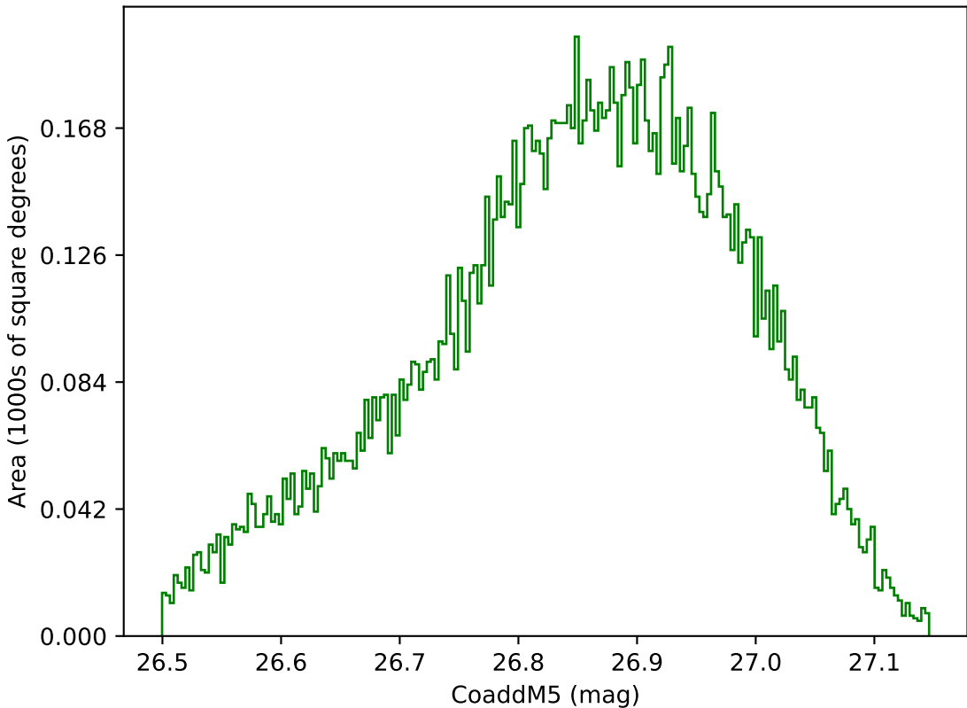
too_elab_2yr_r128_d3_ugrizy_v3.4_10yrs WFD g band: CoaddM5
