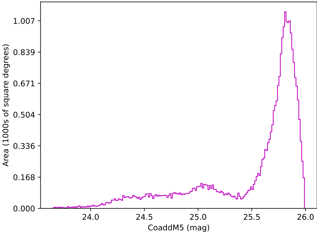
too_elab_2yr_r128_d3_ugrizy_v3.4_10yrs All sky z band: CoaddM5
