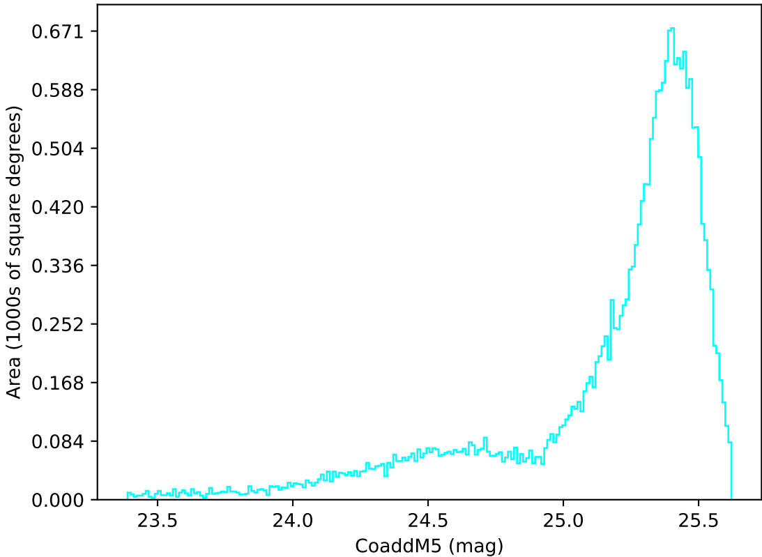
too_elab_2yr_r128_d3_ugrizy_v3.4_10yrs All sky u band: CoaddM5
