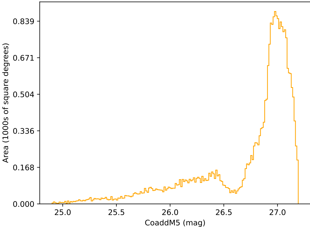
too_elab_2yr_r128_d3_ugrizy_v3.4_10yrs All sky r band: CoaddM5
