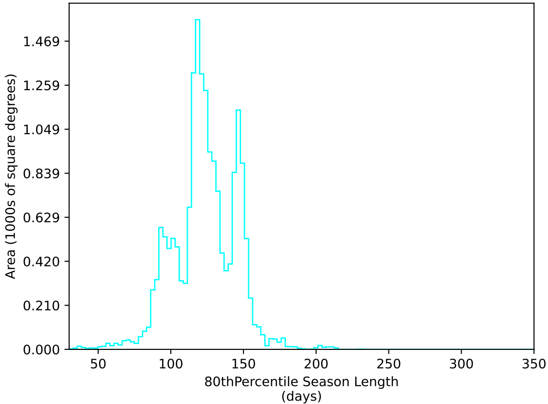
too_elab_2yr_r128_d3_ugrizy_v3.4_10yrs WFD u band: 80thPercentile Season Length
