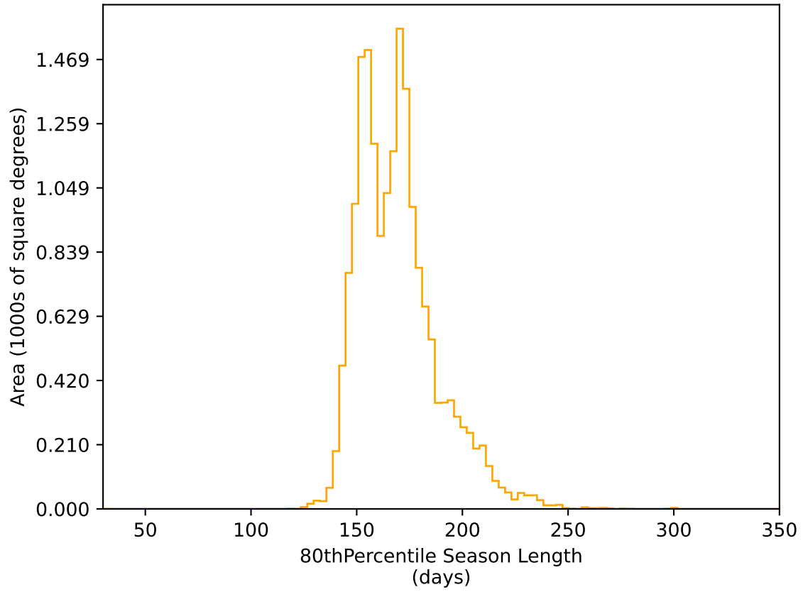
too_elab_2yr_r128_d3_ugrizy_v3.4_10yrs WFD r band: 80thPercentile Season Length
