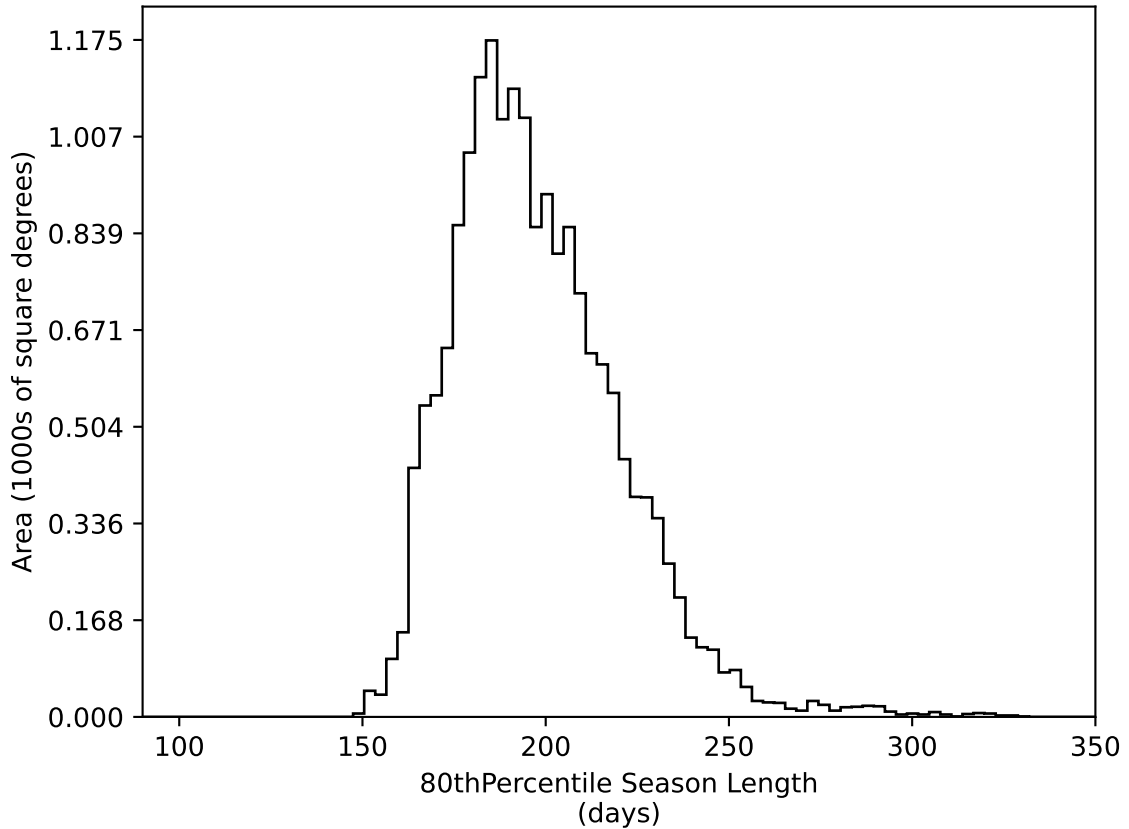
too_elab_2yr_r128_d3_ugrizy_v3.4_10yrs WFD all bands: 80thPercentile Season Length
