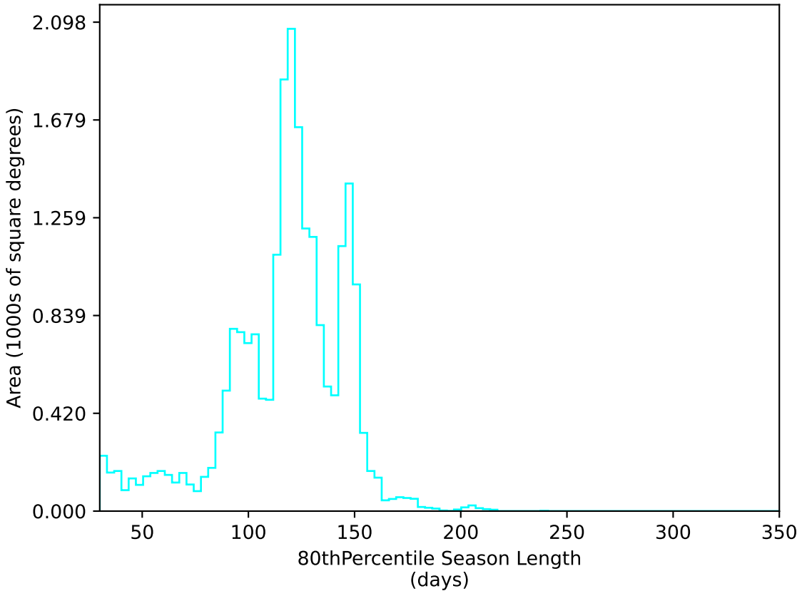
too_elab_2yr_r128_d3_ugrizy_v3.4_10yrs All sky u band: 80thPercentile Season Length
