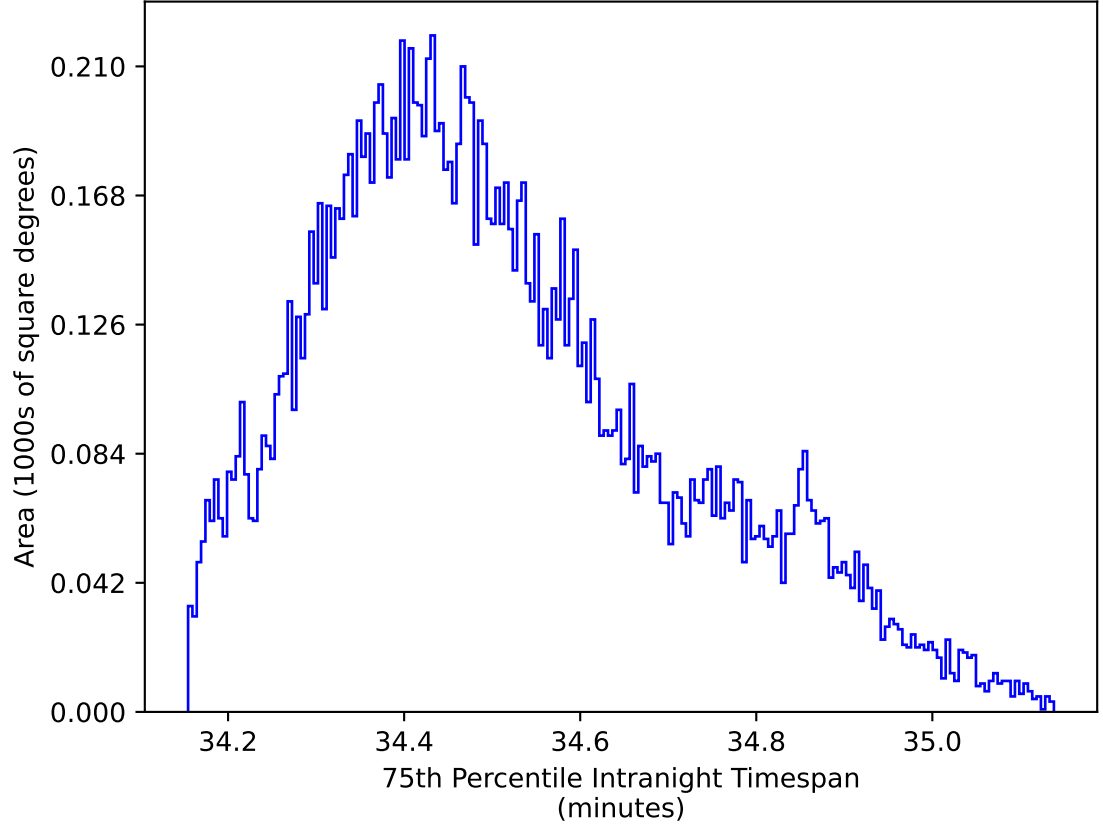
too_elab_2yr_r128_d3_ugrizy_v3.4_10yrs WFD zy bands: 75th Percentile Intranight Timespan
