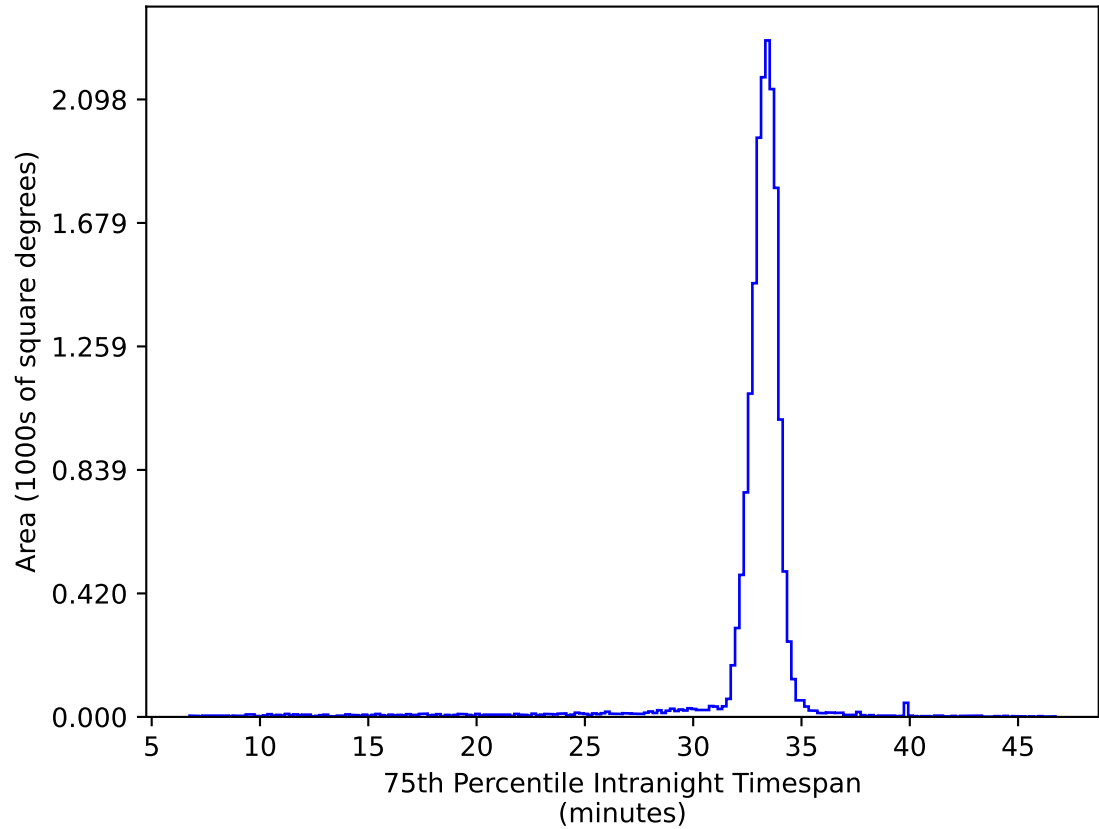
too_elab_2yr_r128_d3_ugrizy_v3.4_10yrs WFD ug bands: 75th Percentile Intranight Timespan
