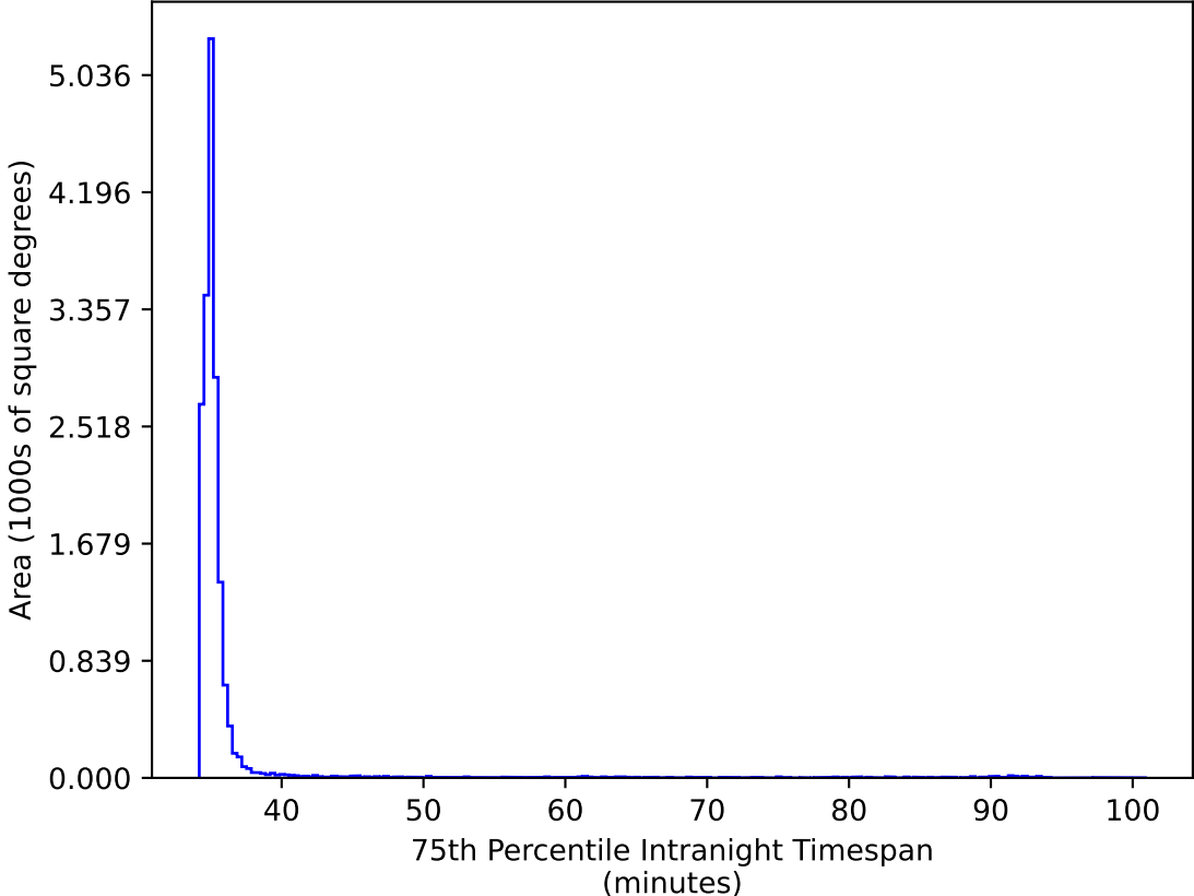
too_elab_2yr_r128_d3_ugrizy_v3.4_10yrs WFD ri bands: 75th Percentile Intranight Timespan
