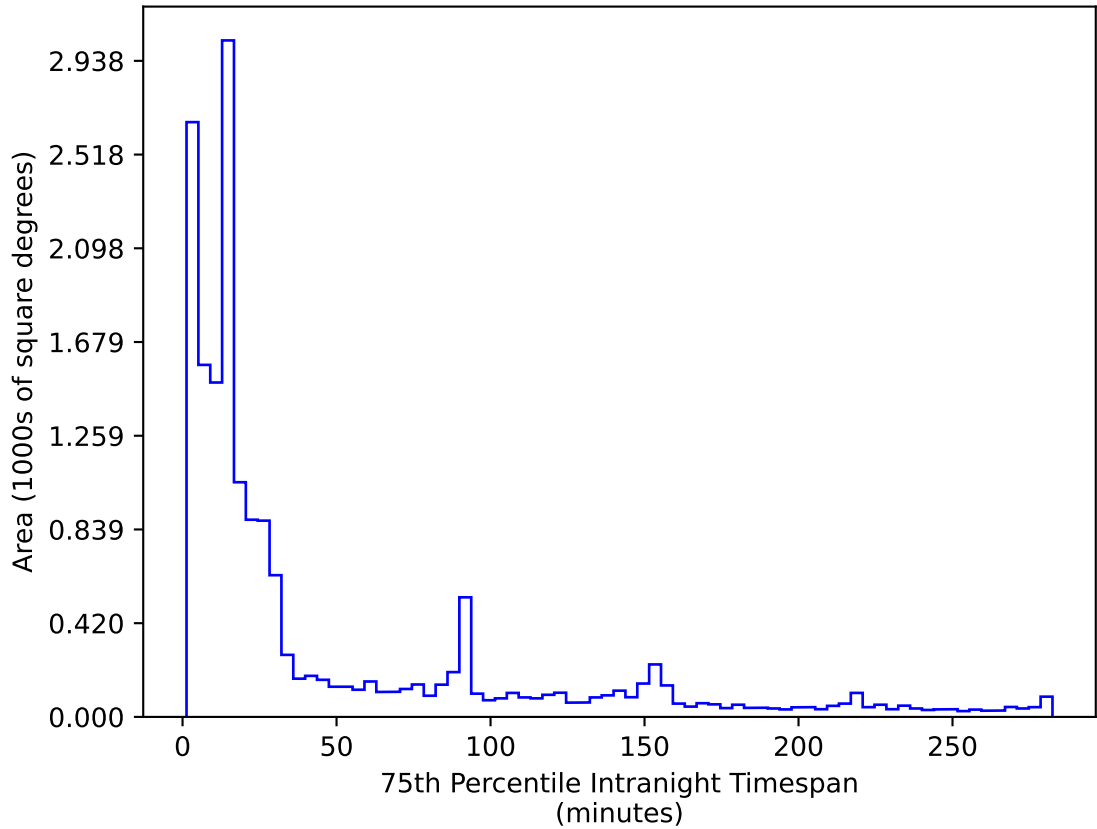
too_elab_2yr_r128_d3_ugrizy_v3.4_10yrs WFD r band: 75th Percentile Intranight Timespan
