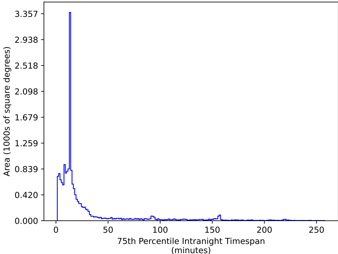
too_elab_2yr_r128_d3_ugrizy_v3.4_10yrs WFD i band: 75th Percentile Intranight Timespan
