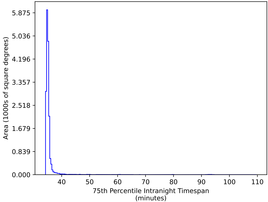
too_elab_2yr_r128_d3_ugrizy_v3.4_10yrs WFD gr bands: 75th Percentile Intranight Timespan
