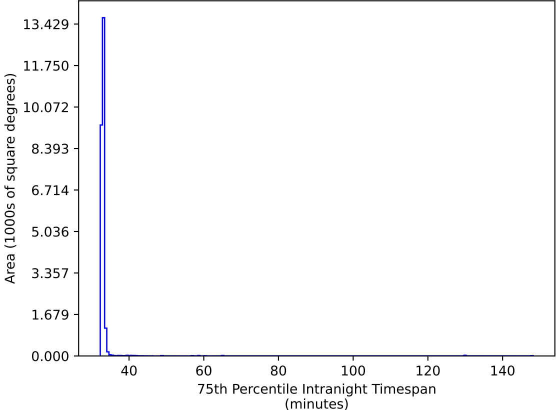
too_elab_2yr_r128_d3_ugrizy_v3.4_10yrs All sky y band: 75th Percentile Intranight Timespan
