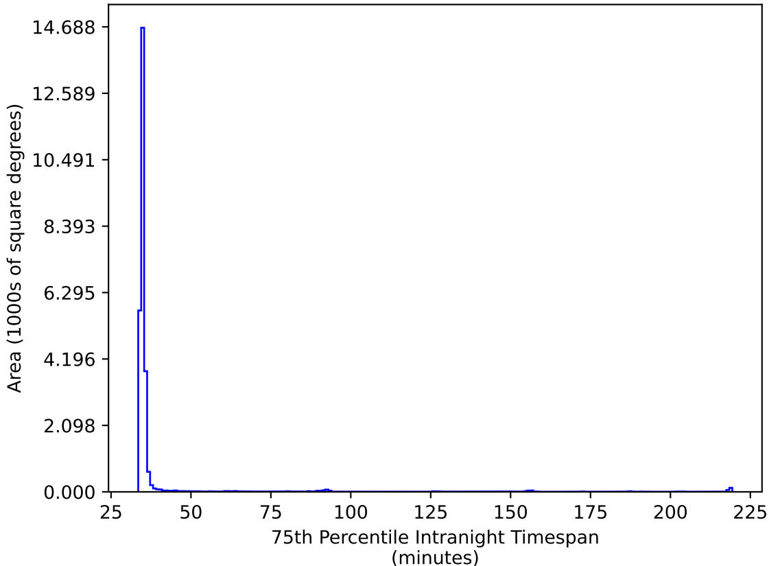
too_elab_2yr_r128_d3_ugrizy_v3.4_10yrs All sky ri bands: 75th Percentile Intranight Timespan
