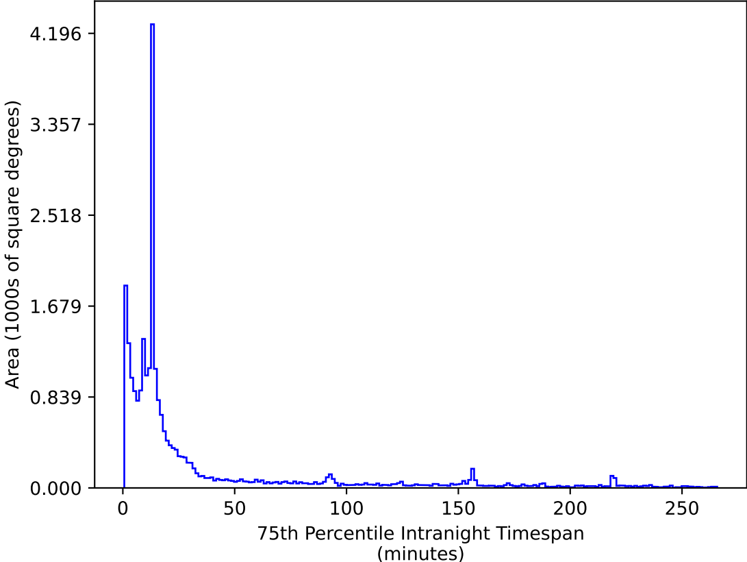
too_elab_2yr_r128_d3_ugrizy_v3.4_10yrs All sky i band: 75th Percentile Intranight Timespan
