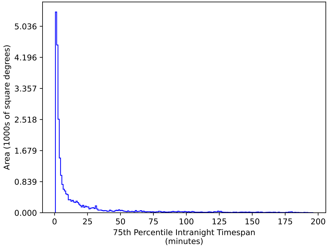
too_elab_2yr_r128_d3_ugrizy_v3.4_10yrs All sky g band: 75th Percentile Intranight Timespan
