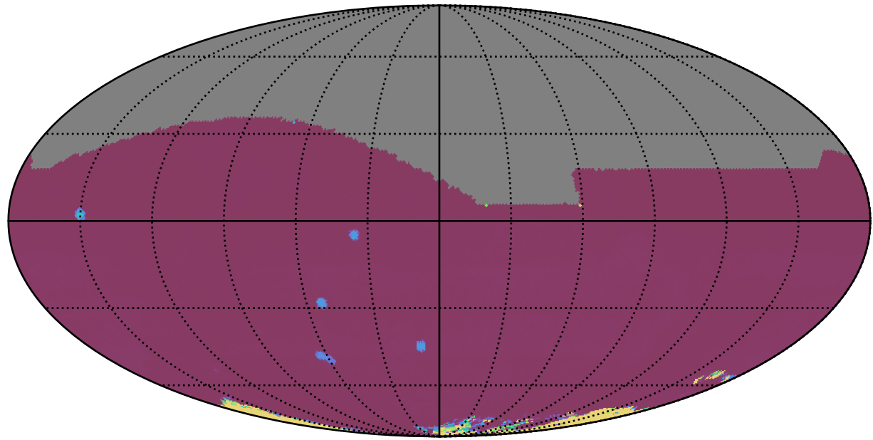
too_elab_2yr_r128_d3_ugrizy_v3.4_10yrs All sky all bands: 75th Percentile Intranight Timespan
