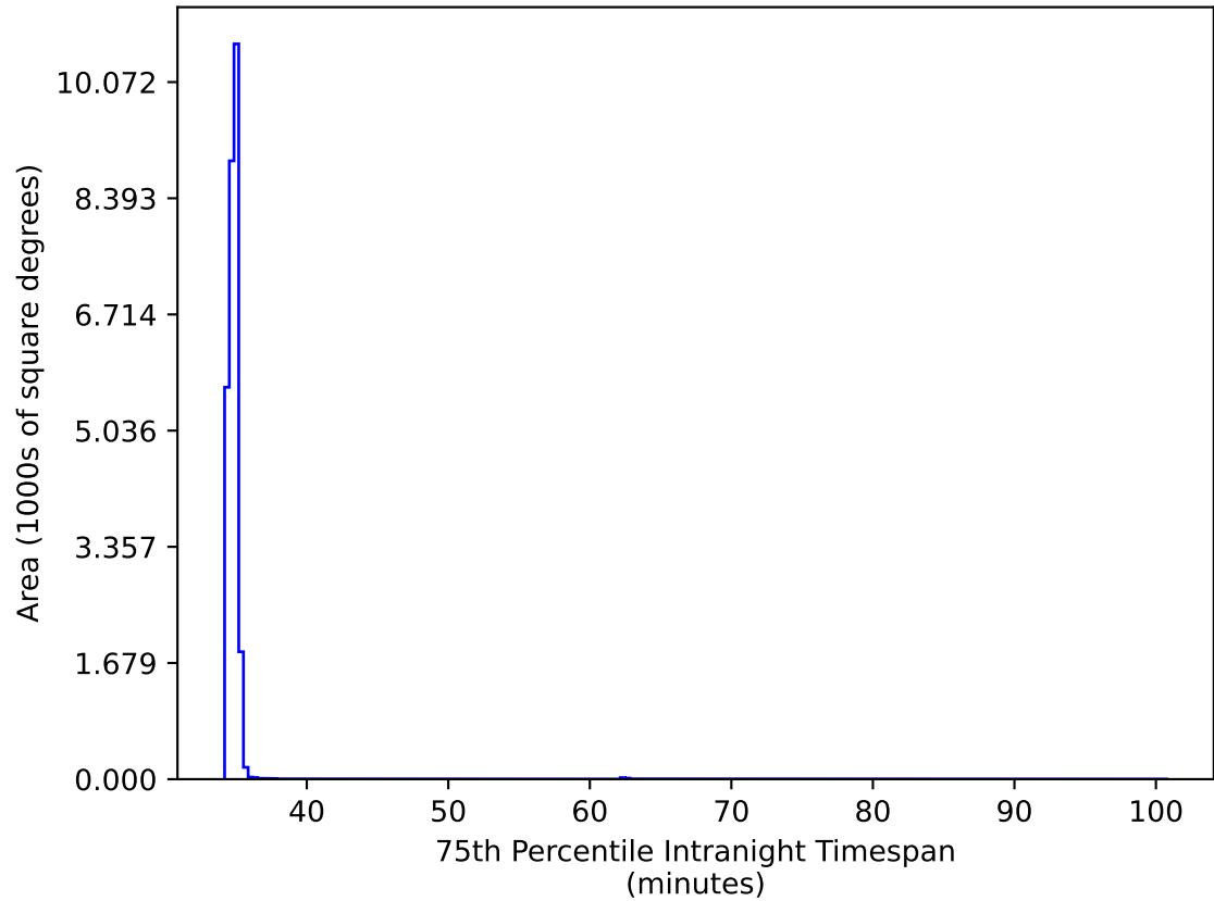
too_elab_2yr_r128_d3_ugrizy_v3.4_10yrs All sky: 75th Percentile Intranight Timespan
